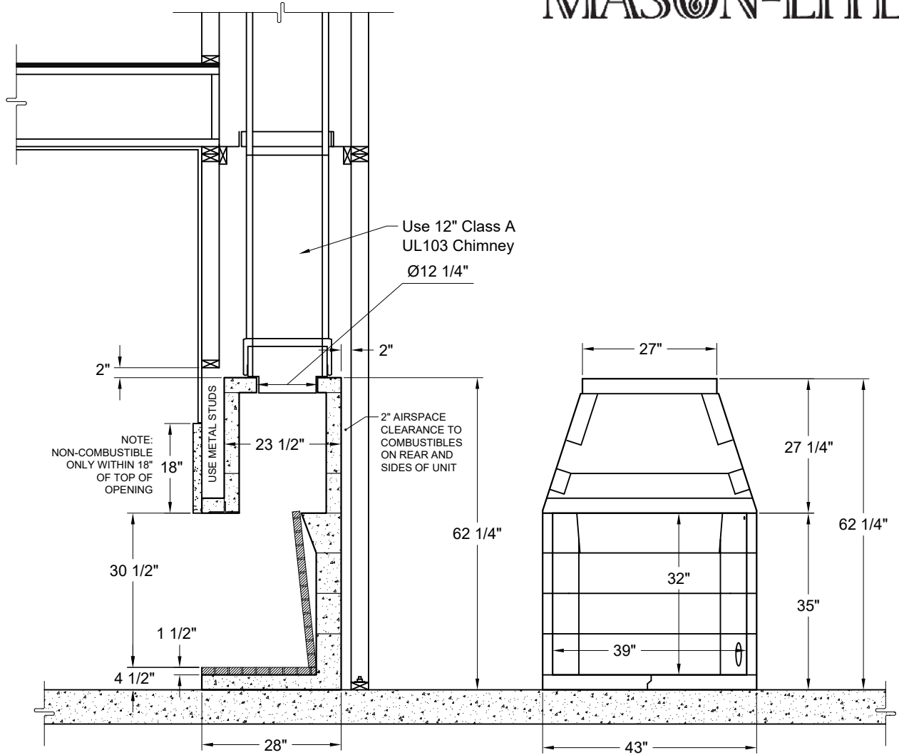
SECTION
