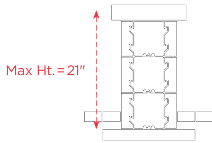
Seat Walls
