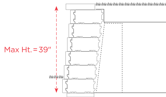
Walls (24" - 39")
